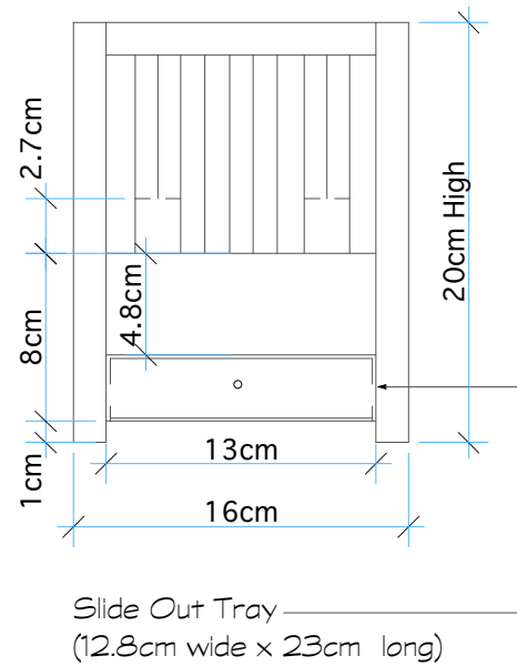
END VIEW
